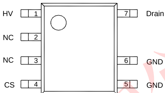
SOP-7
